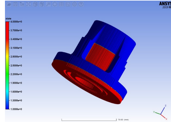
3D Printing simulation showing support in red color
