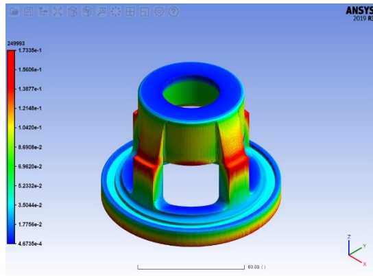
3D Printing thermal deformation simulation
