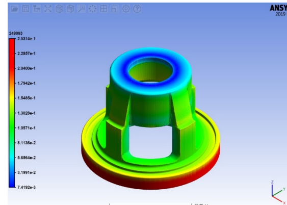
3D Printing simulation after design compensation of thermal deformation
